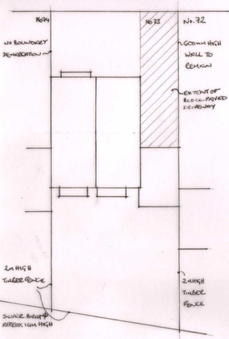
EXISTING SITE AND ROOF PLAN 1:200
